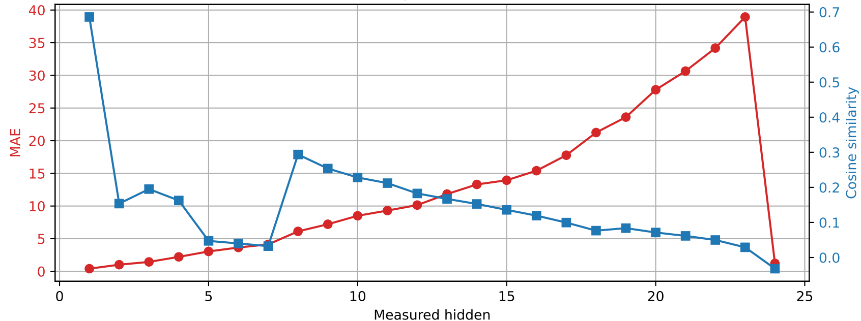
SmolLM2-1.7B-Instruct | Prompt 3 Spared layer 17 | Unquantized vs hybrid
