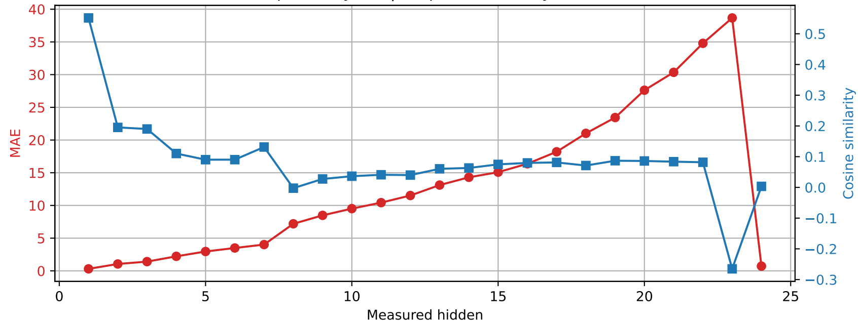
SmolLM2-1.7B-Instruct | Prompt 4 Spared layer 2 | Unquantized vs hybrid
