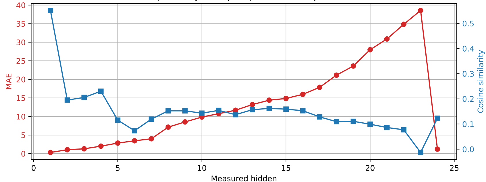
SmolLM2-1.7B-Instruct | Prompt 4 Spared layer 12 | Unquantized vs hybrid
