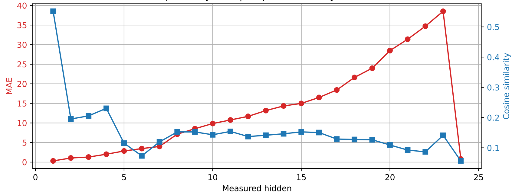
SmolLM2-1.7B-Instruct | Prompt 4 Spared layer 16 | Unquantized vs hybrid
