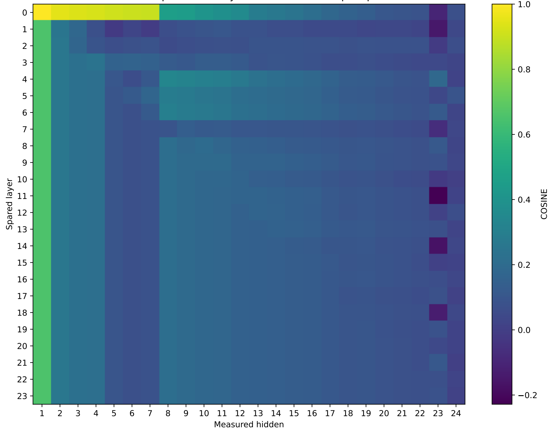
SmolLM2-1.7B-Instruct Mean unquantized vs hybrid cos sim across 5 prompts
