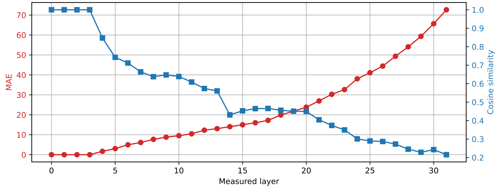
SmolLM2-360M | Prompt 0 Spared layer 3 | Hybrid vs quantized
