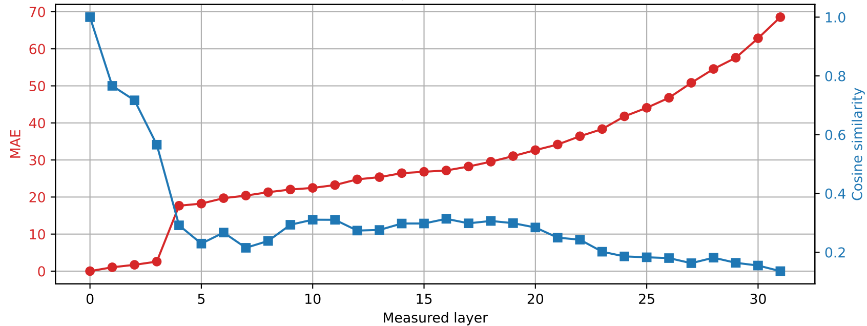
SmolLM2-360M | Prompt 0 Spared layer 3 | Hybrid vs unquantized
