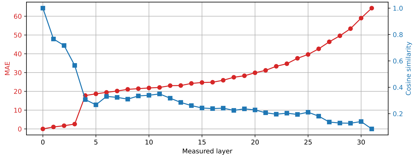
SmolLM2-360M | Prompt 0 Spared layer 5 | Hybrid vs unquantized
