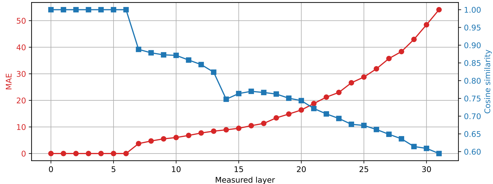
SmolLM2-360M | Prompt 0 Spared layer 6 | Hybrid vs quantized
