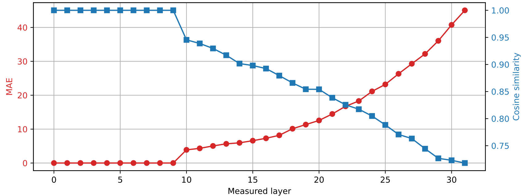
SmolLM2-360M | Prompt 0 Spared layer 9 | Hybrid vs quantized
