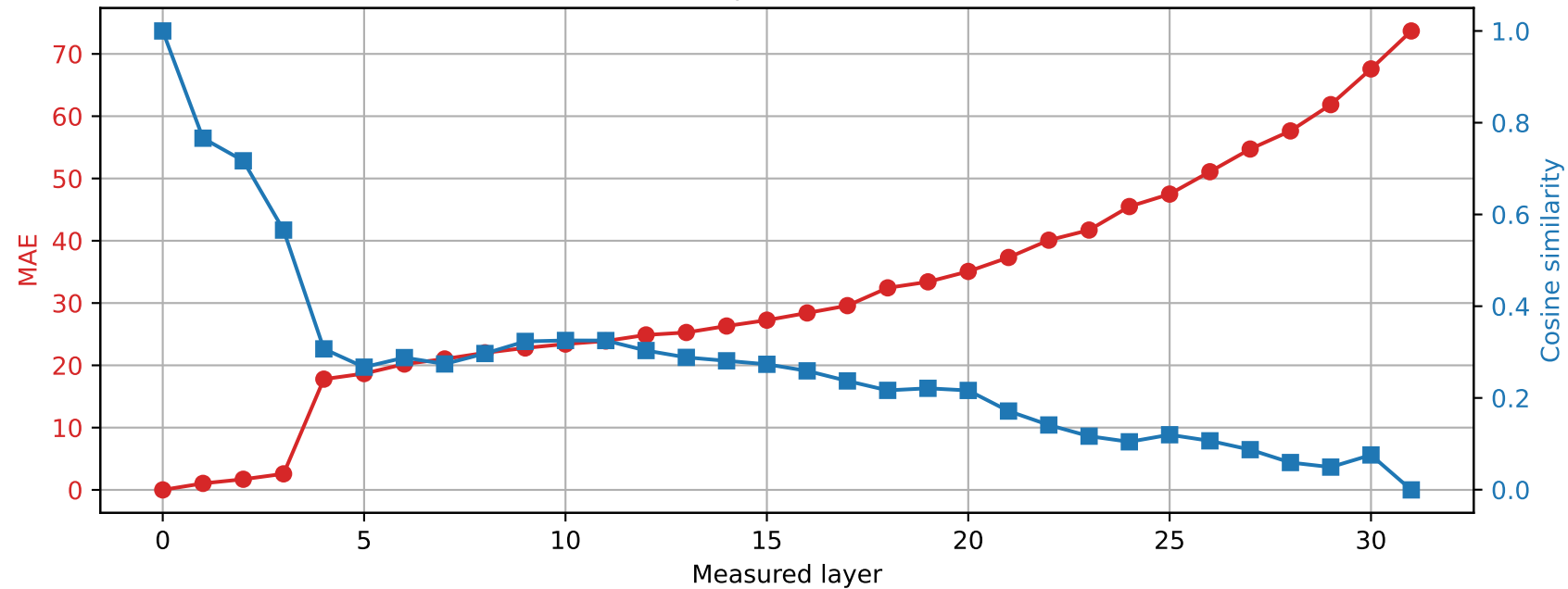
SmolLM2-360M | Prompt 0 Spared layer 18 | Hybrid vs unquantized
