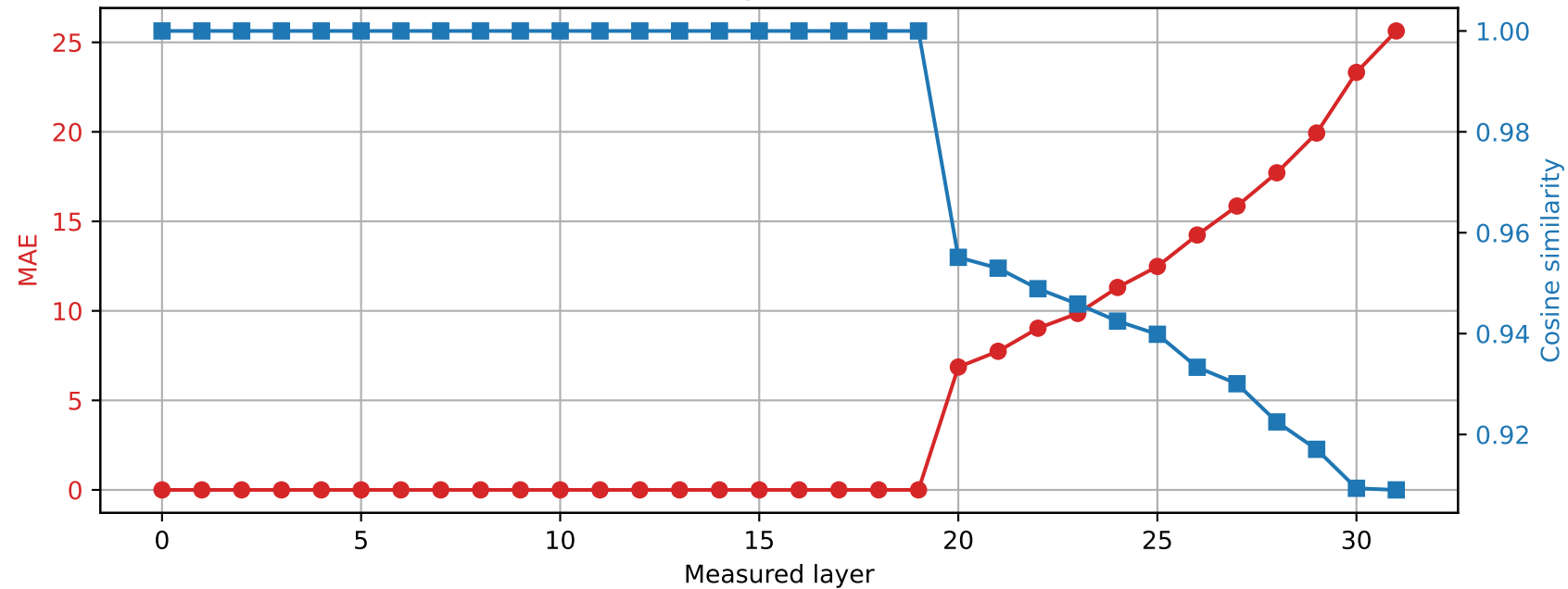
SmolLM2-360M | Prompt 0 Spared layer 19 | Hybrid vs quantized
