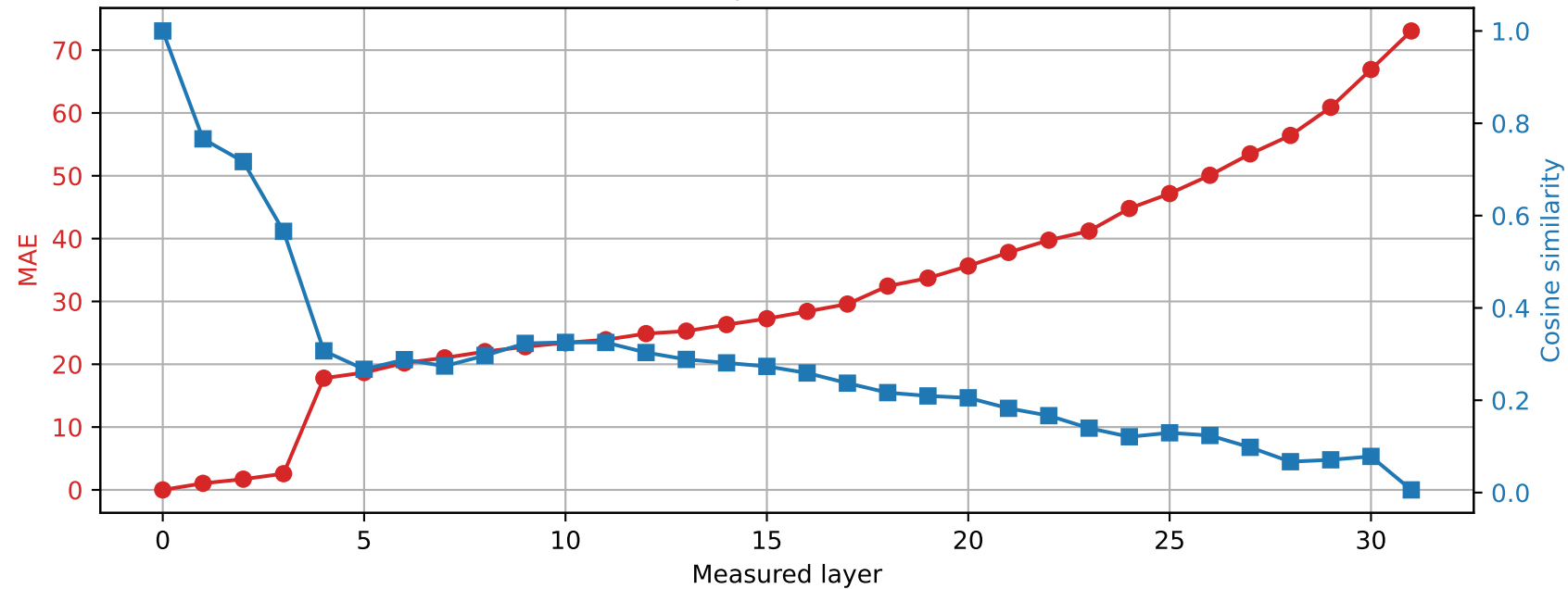
SmolLM2-360M | Prompt 0 Spared layer 21 | Hybrid vs unquantized
