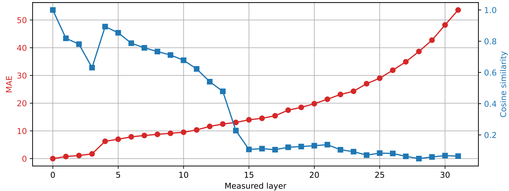
SmolLM2-360M | Prompt 1 Unquantized vs quantized int4
