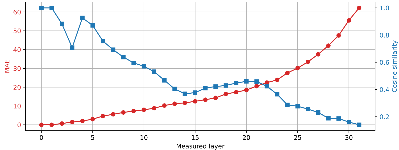
SmolLM2-360M | Prompt 1 Spared layer 1 | Hybrid vs quantized
