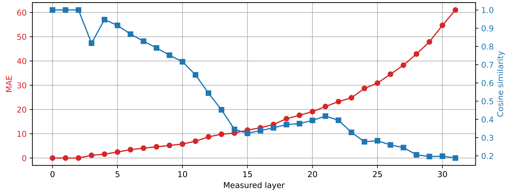
SmolLM2-360M | Prompt 1 Spared layer 2 | Hybrid vs quantized
