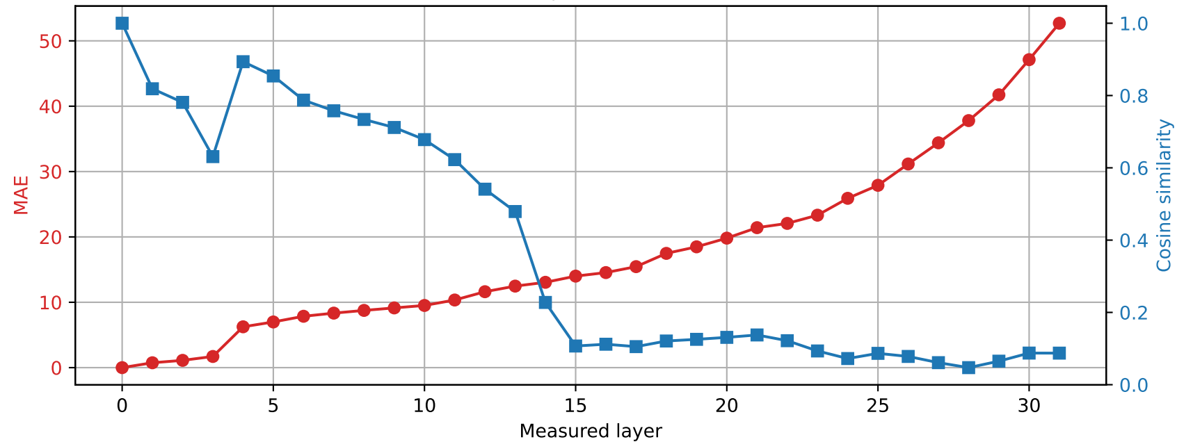
SmolLM2-360M | Prompt 1 Spared layer 21 | Hybrid vs unquantized
