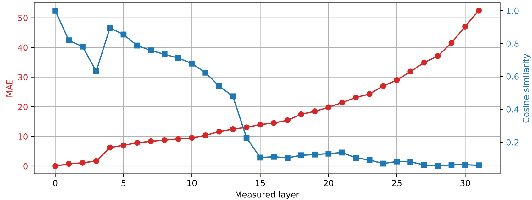
SmolLM2-360M | Prompt 1 Spared layer 27 | Hybrid vs unquantized
