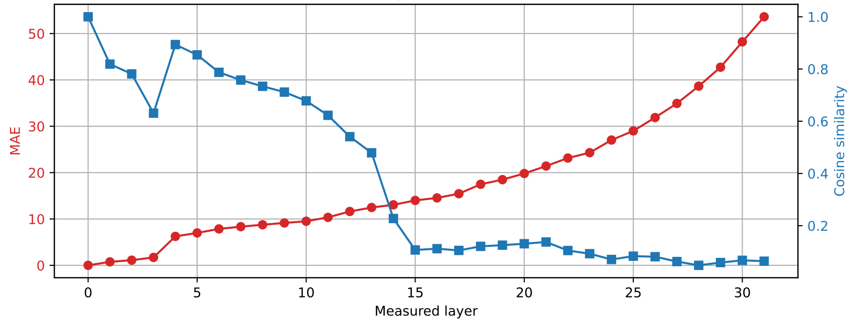
SmolLM2-360M | Prompt 1 Spared layer 31 | Hybrid vs unquantized
