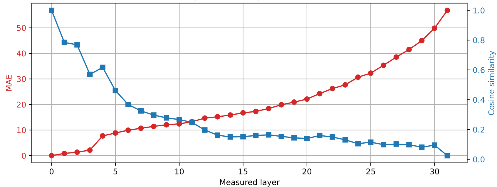
SmolLM2-360M | Prompt 2 Unquantized vs quantized int4
