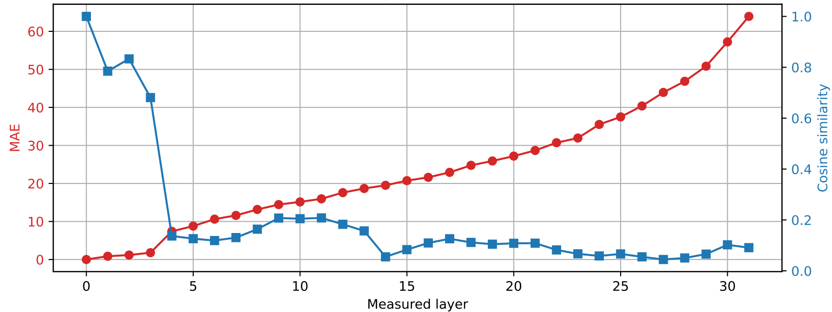
SmolLM2-360M | Prompt 2 Spared layer 1 | Hybrid vs unquantized
