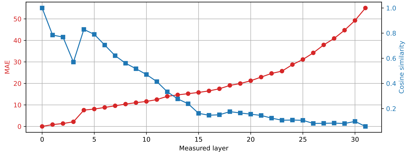
SmolLM2-360M | Prompt 2 Spared layer 3 | Hybrid vs unquantized
