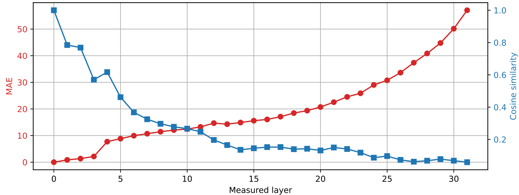
SmolLM2-360M | Prompt 2 Spared layer 12 | Hybrid vs unquantized
