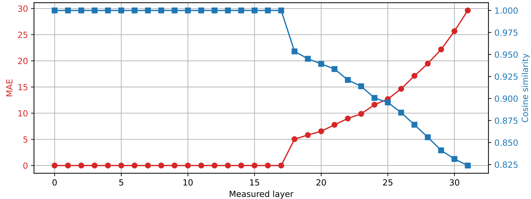
SmolLM2-360M | Prompt 2 Spared layer 17 | Hybrid vs quantized
