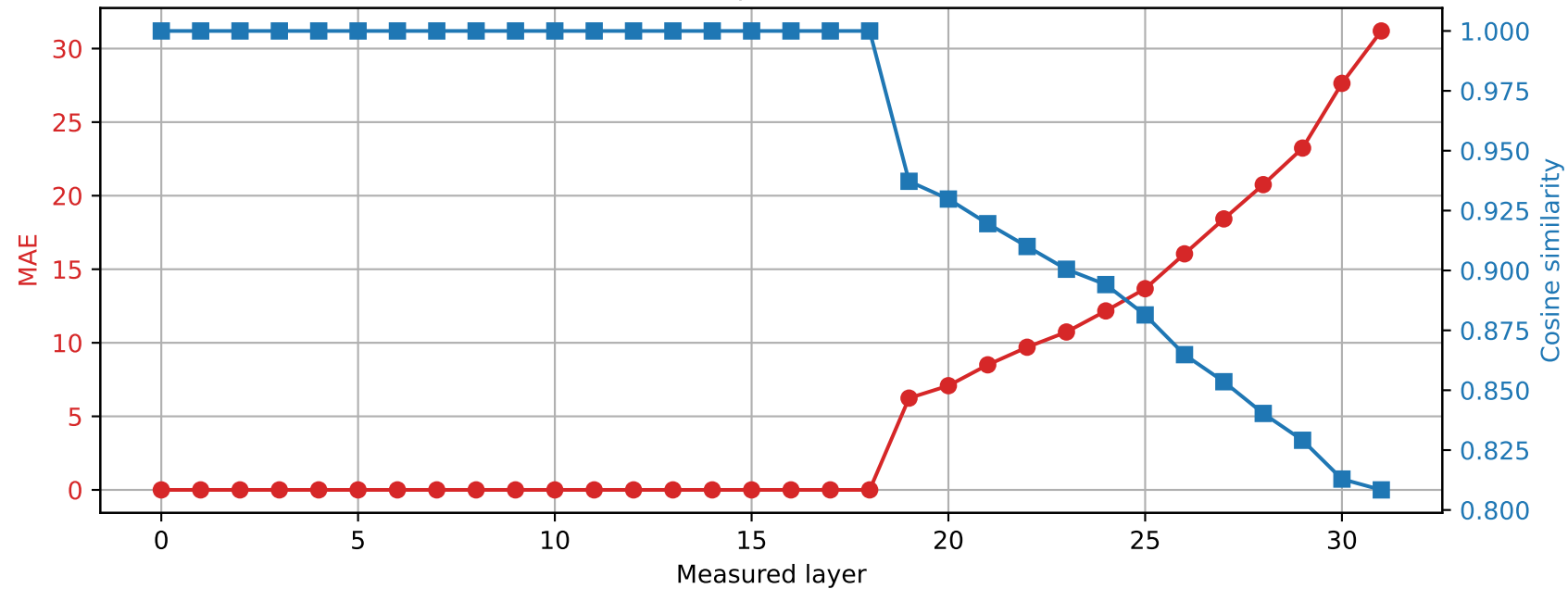
SmolLM2-360M | Prompt 2 Spared layer 18 | Hybrid vs quantized
