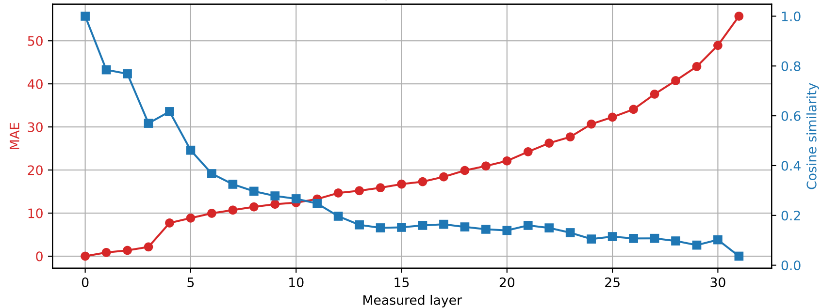
SmolLM2-360M | Prompt 2 Spared layer 25 | Hybrid vs unquantized
