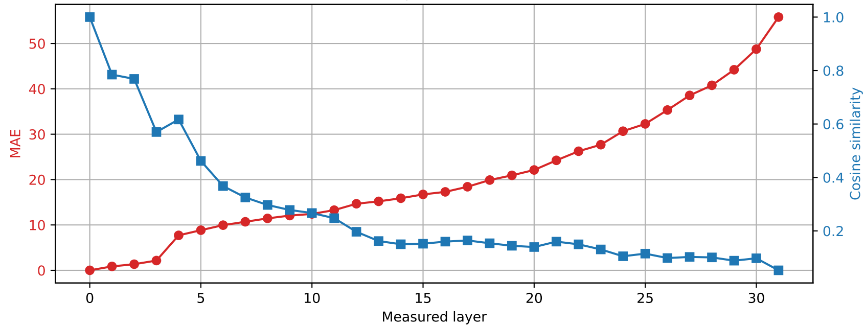
SmolLM2-360M | Prompt 2 Spared layer 27 | Hybrid vs unquantized
