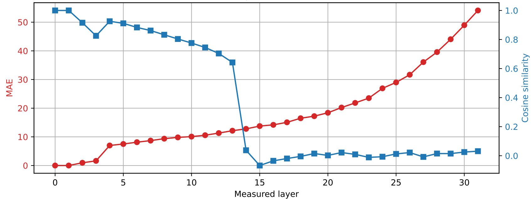
SmolLM2-360M | Prompt 3 Spared layer 0 | Hybrid vs unquantized
