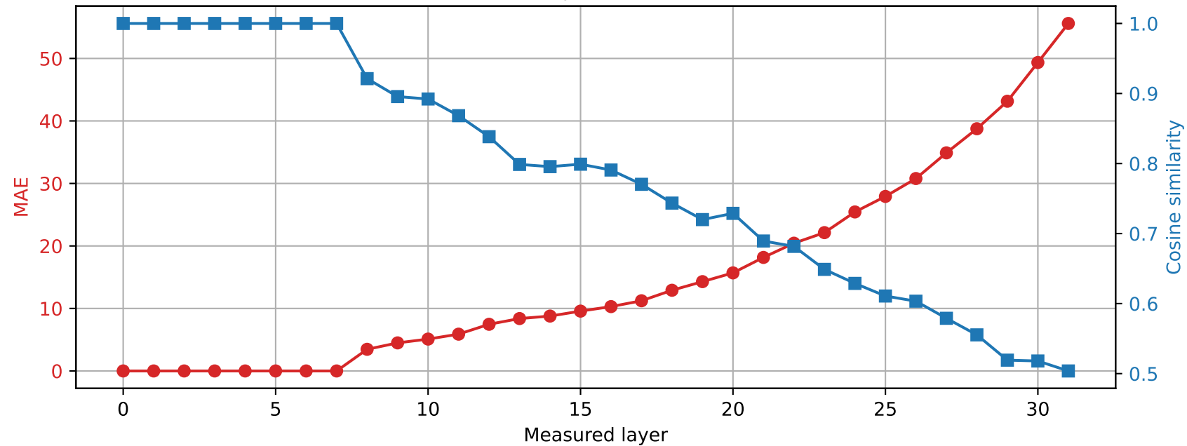
SmolLM2-360M | Prompt 3 Spared layer 7 | Hybrid vs quantized
