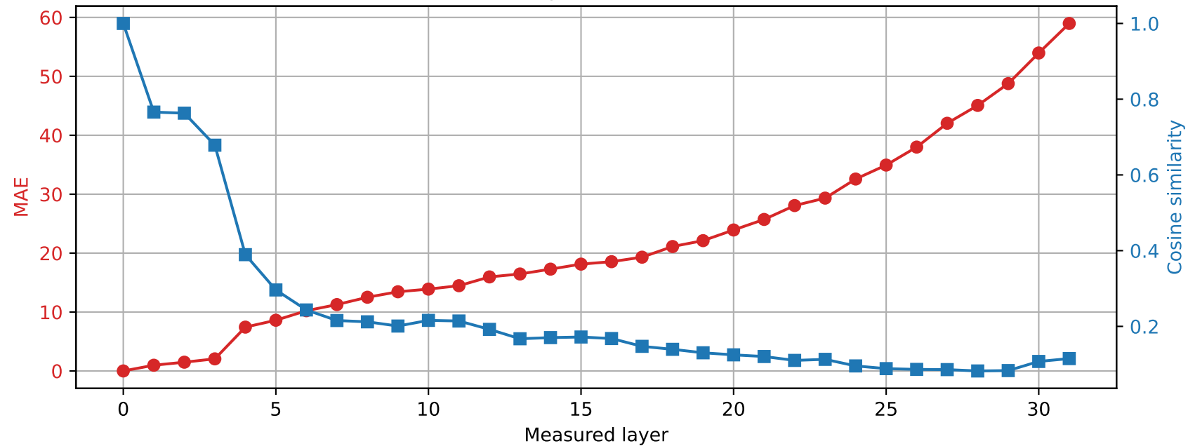
SmolLM2-360M | Prompt 3 Spared layer 8 | Hybrid vs unquantized
