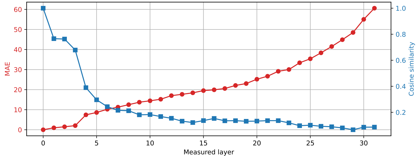
SmolLM2-360M | Prompt 3 Spared layer 14 | Hybrid vs unquantized
