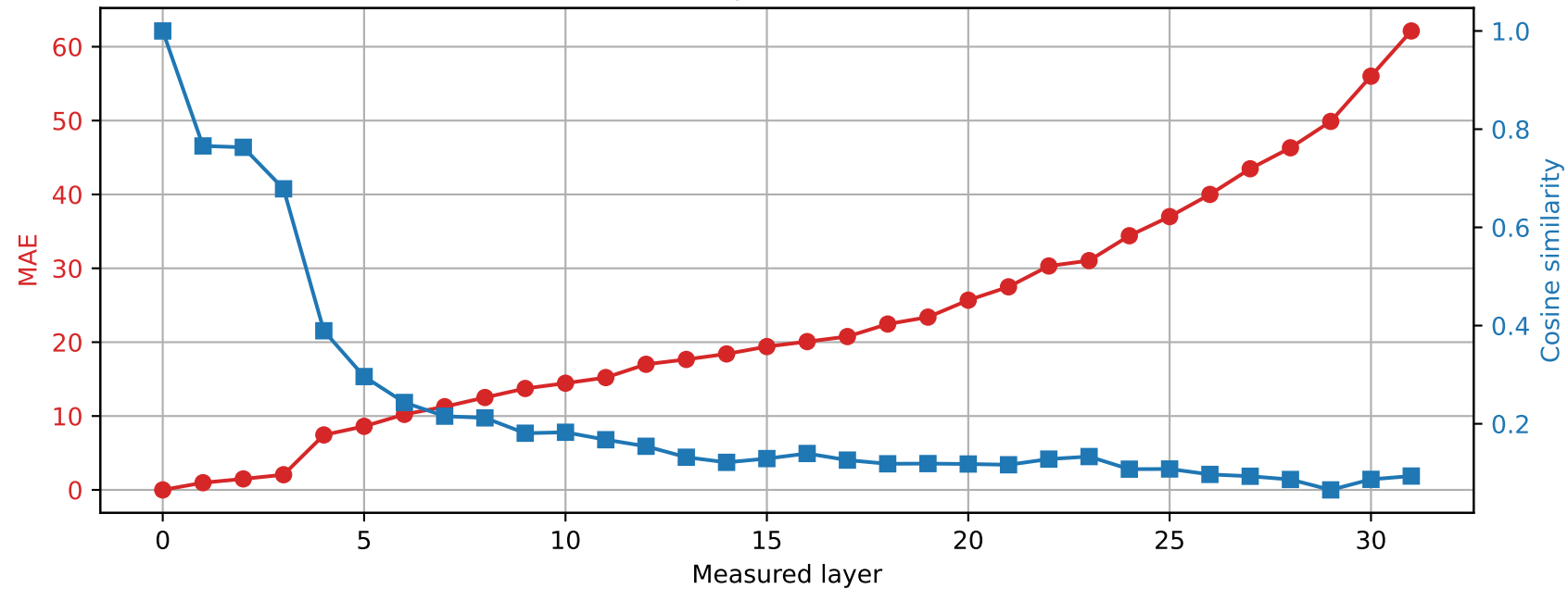
SmolLM2-360M | Prompt 3 Spared layer 22 | Hybrid vs unquantized
