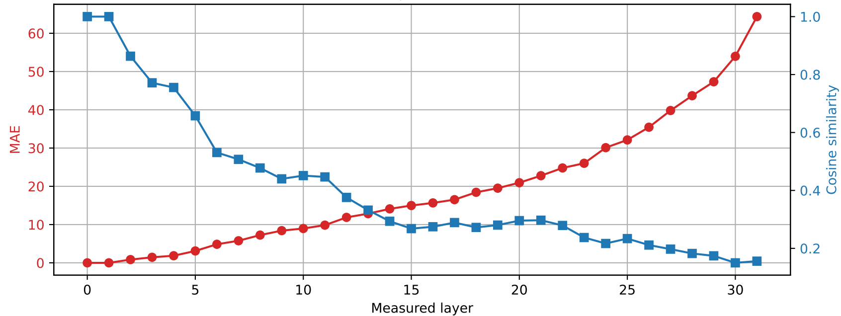
SmolLM2-360M | Prompt 4 Spared layer 1 | Hybrid vs quantized
