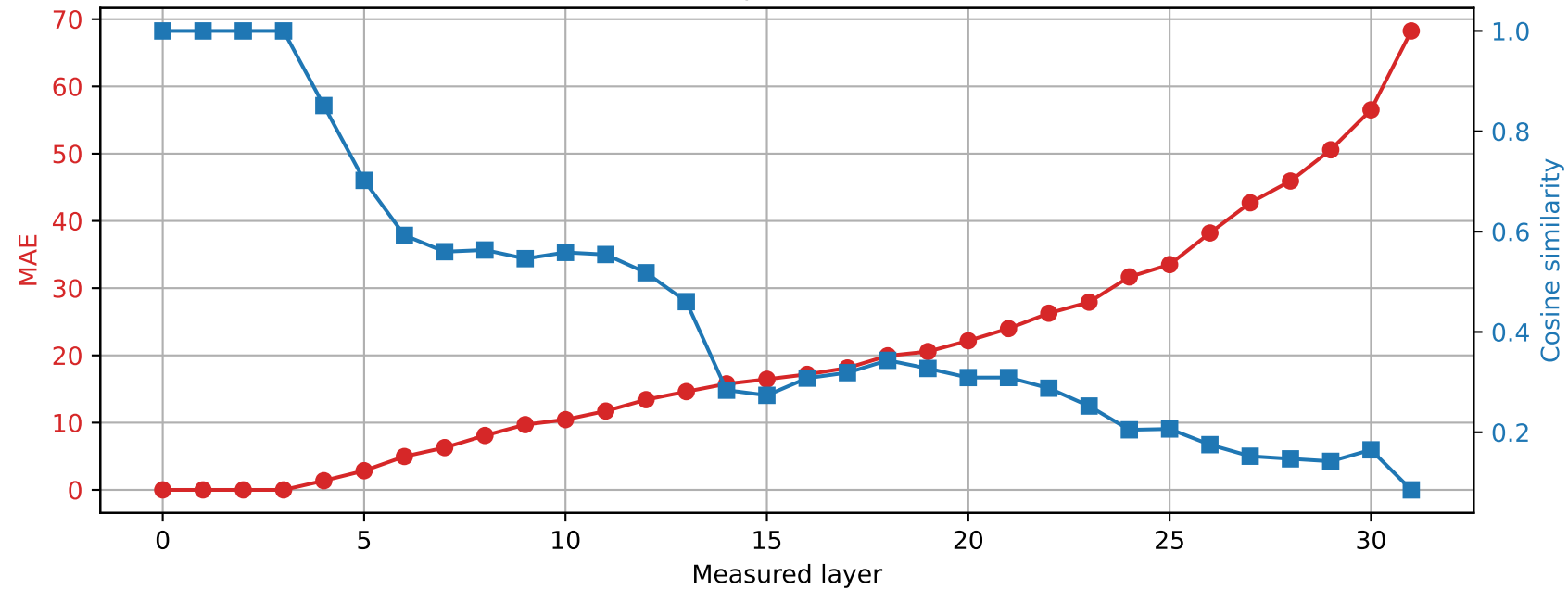
SmolLM2-360M | Prompt 4 Spared layer 3 | Hybrid vs quantized
