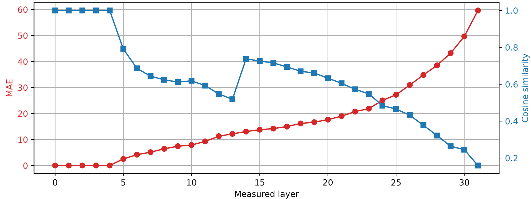
SmolLM2-360M | Prompt 4 Spared layer 4 | Hybrid vs quantized
