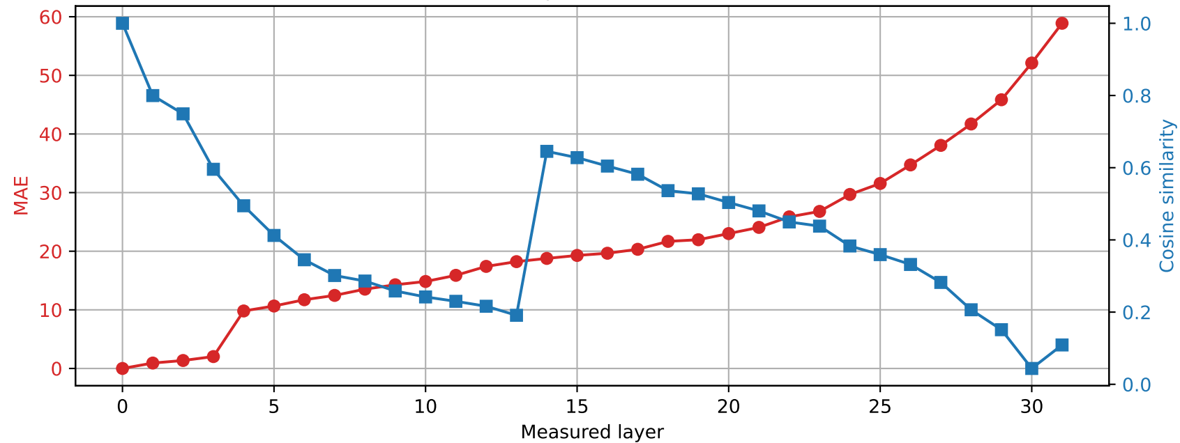
SmolLM2-360M | Prompt 4 Spared layer 4 | Hybrid vs unquantized
