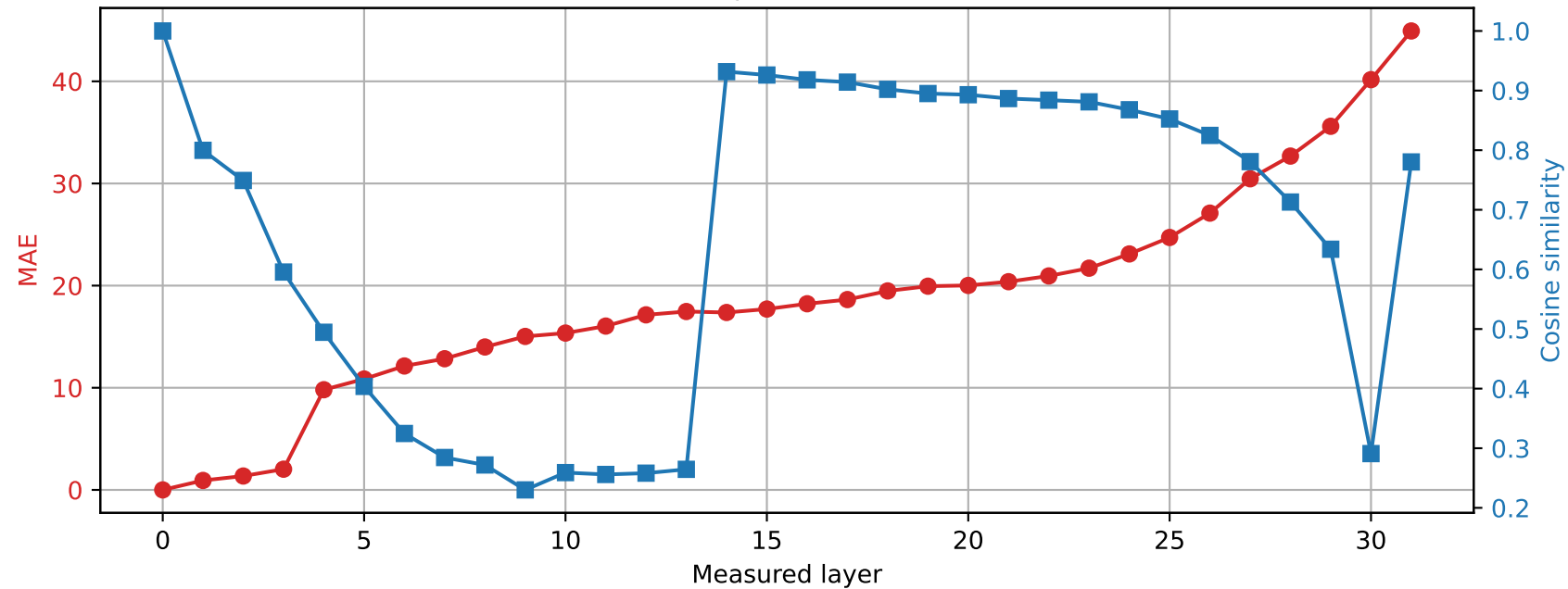
SmolLM2-360M | Prompt 4 Spared layer 19 | Hybrid vs unquantized
