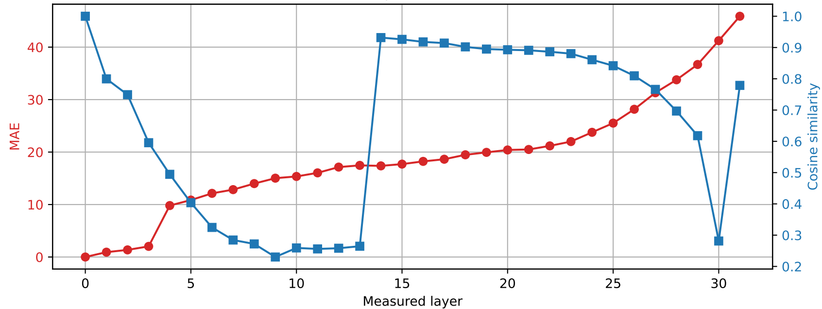
SmolLM2-360M | Prompt 4 Spared layer 20 | Hybrid vs unquantized
