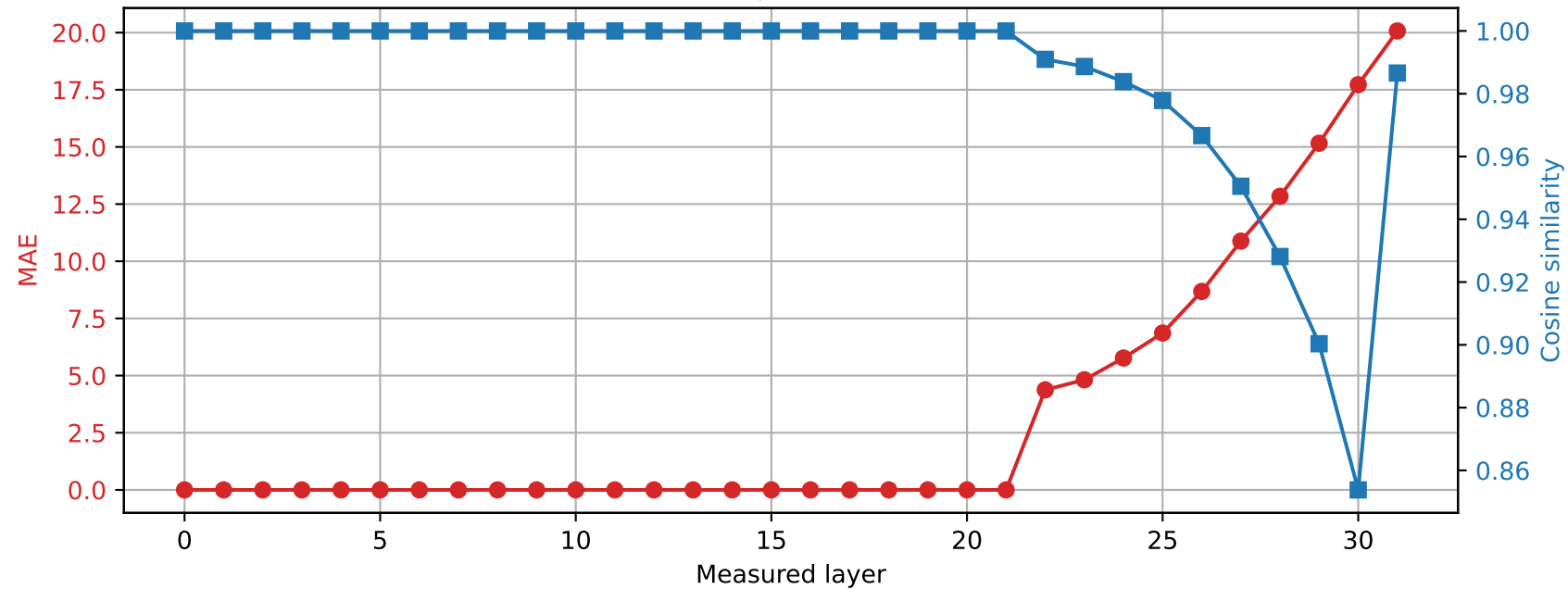
SmolLM2-360M | Prompt 4 Spared layer 21 | Hybrid vs quantized
