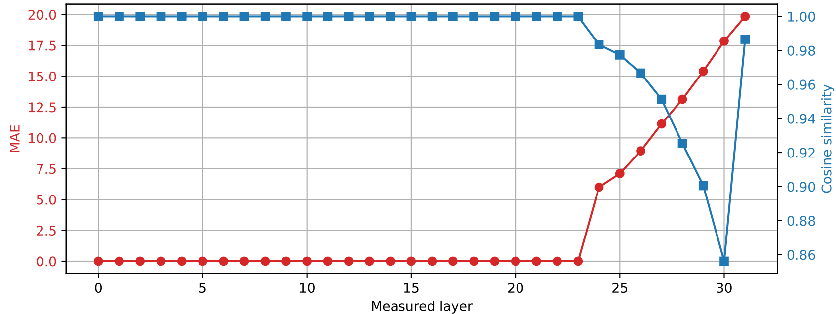
SmolLM2-360M | Prompt 4 Spared layer 23 | Hybrid vs quantized
