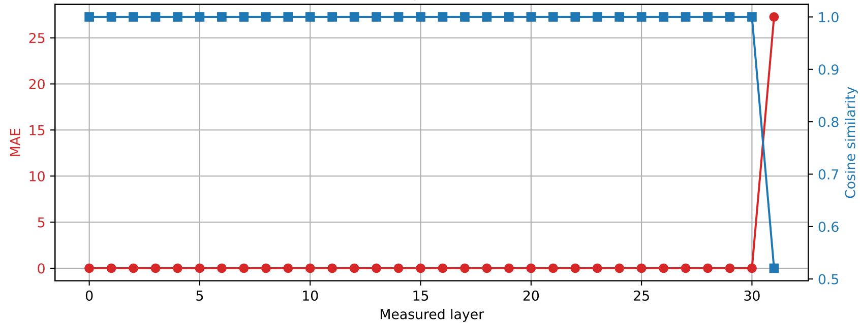
SmolLM2-360M | Prompt 4 Spared layer 30 | Hybrid vs quantized
