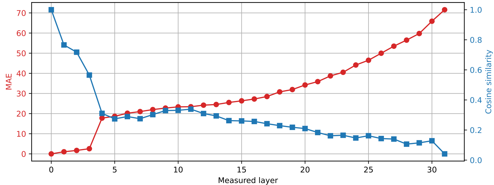
SmolLM2-360M | Prompt 0 Spared layer 10 | Hybrid vs unquantized
