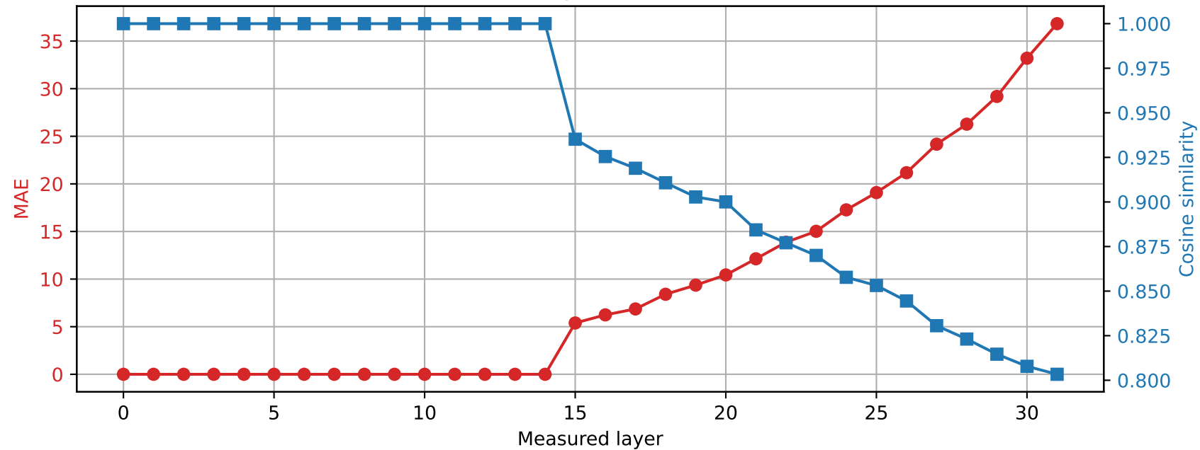
SmolLM2-360M | Prompt 0 Spared layer 14 | Hybrid vs quantized
