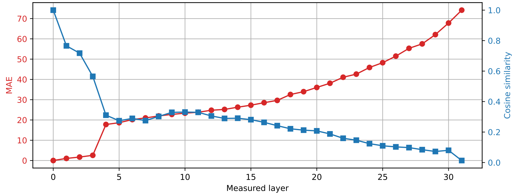
SmolLM2-360M | Prompt 0 Spared layer 22 | Hybrid vs unquantized
