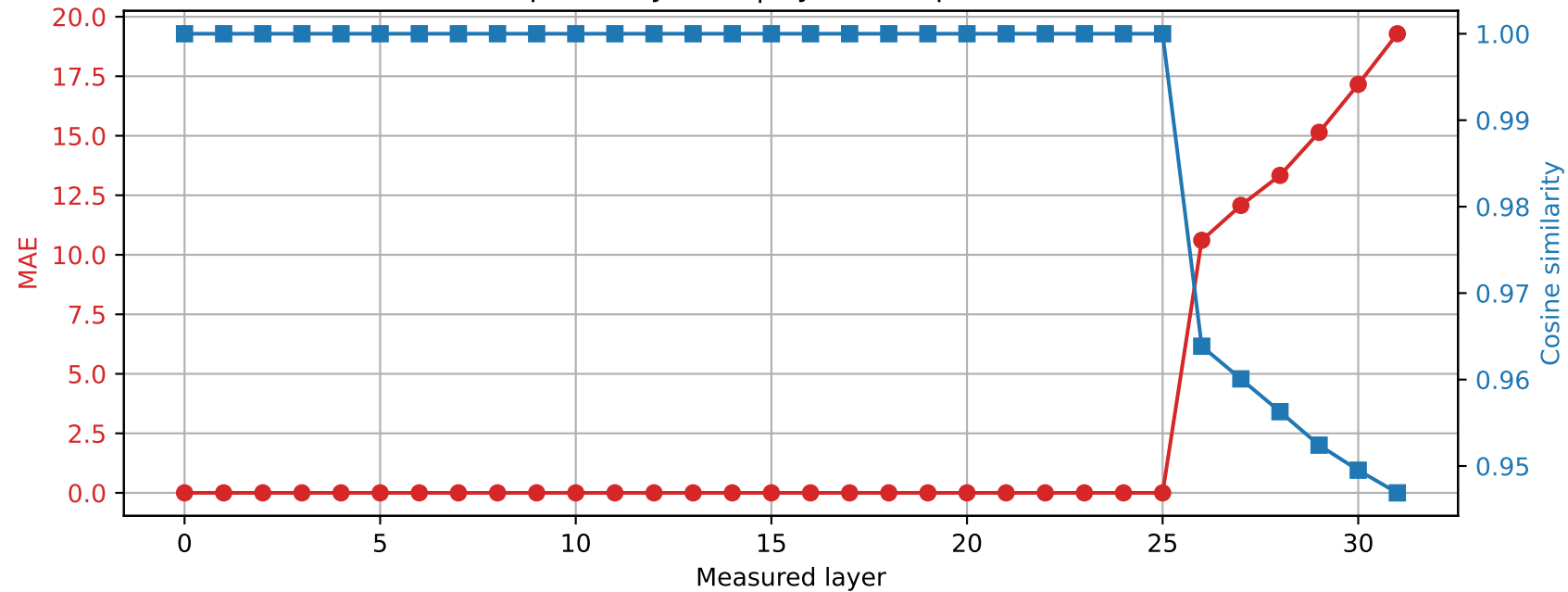
SmolLM2-360M | Prompt 0 Spared layer 25 | Hybrid vs quantized
