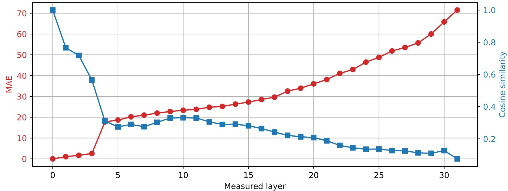
SmolLM2-360M | Prompt 0 Spared layer 26 | Hybrid vs unquantized
