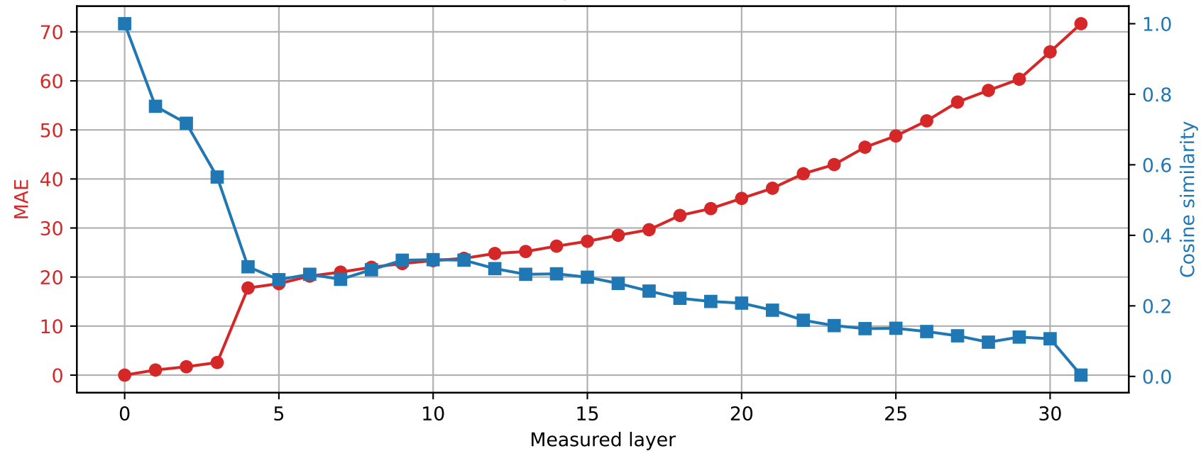
SmolLM2-360M | Prompt 0 Spared layer 28 | Hybrid vs unquantized
