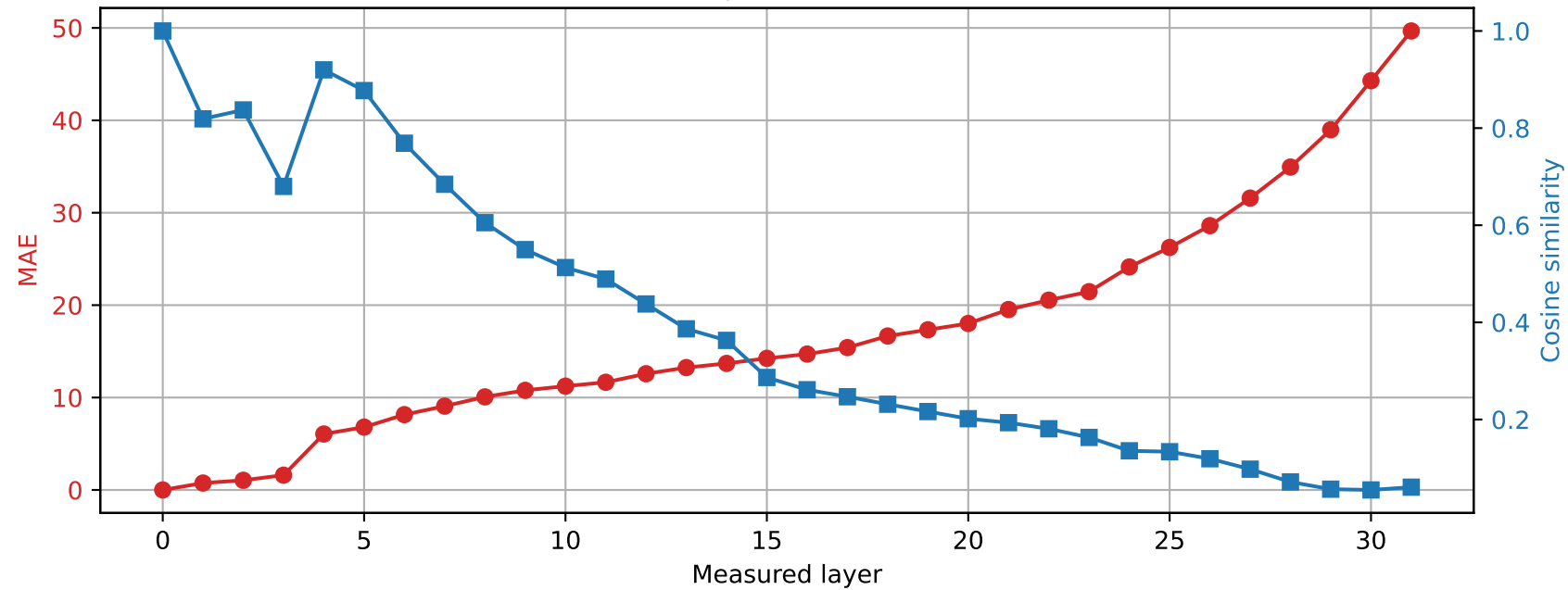
SmolLM2-360M | Prompt 1 Spared layer 1 | Hybrid vs unquantized
