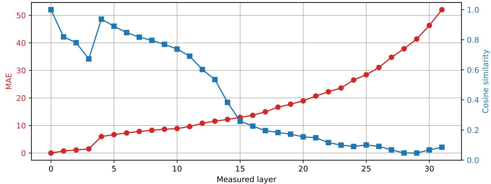
SmolLM2-360M | Prompt 1 Spared layer 2 | Hybrid vs unquantized
