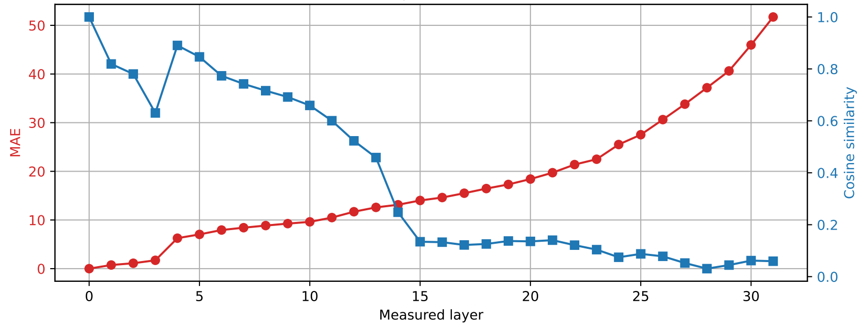
SmolLM2-360M | Prompt 1 Spared layer 17 | Hybrid vs unquantized
